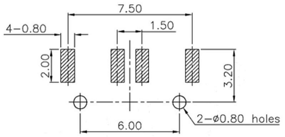
PCB Layout (Pattern side)
